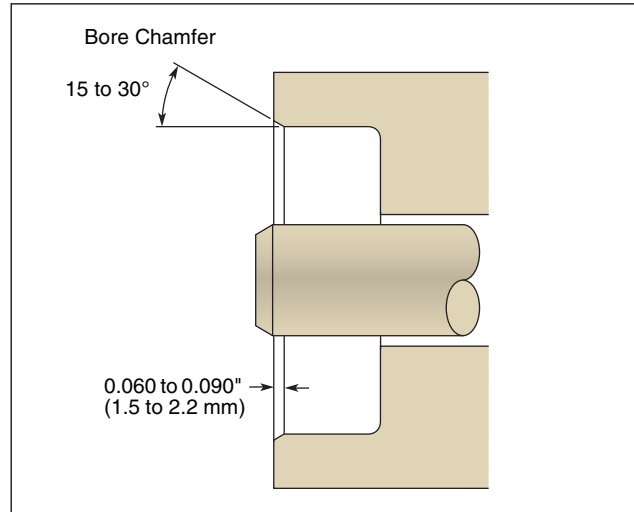
Figure 2-10. Housing Profile
