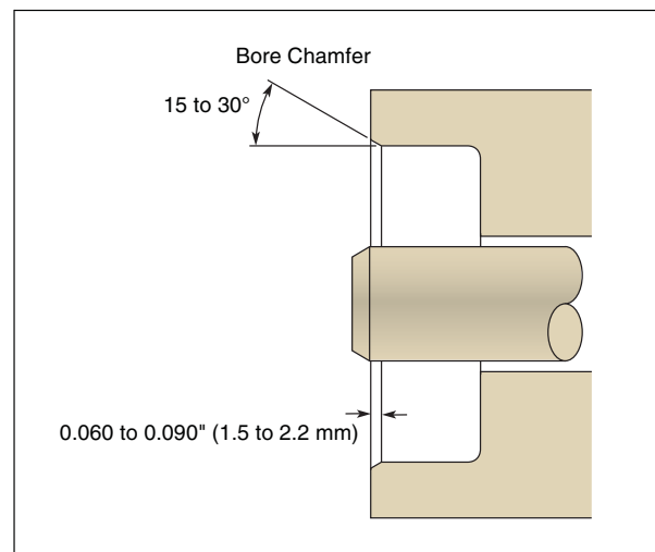
Figure 6-2. Housing Profile
