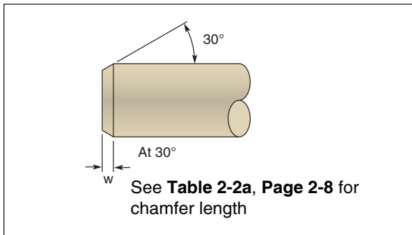
Figure 6-1. Shaft Profile
