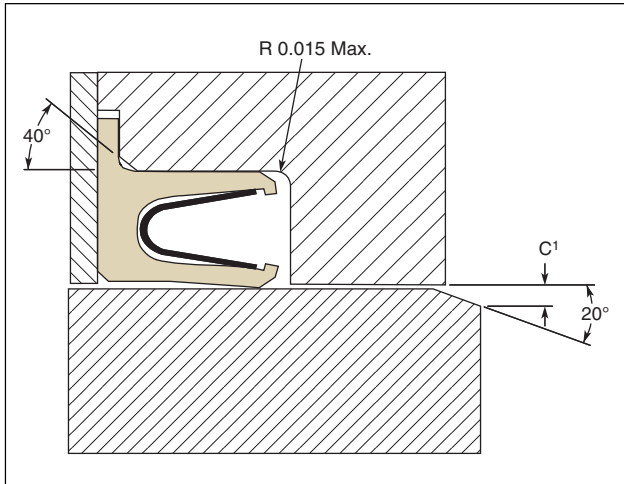
Figure 2-20. Two-Piece Flanged Gland
