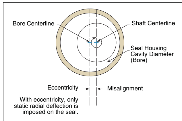
Figure 2-11. STBM
