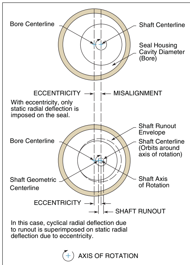
Figure 2-22. Eccentricity and Shaft Runout
