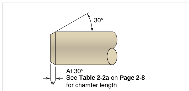
Figure 2-18. Shaft Profile
