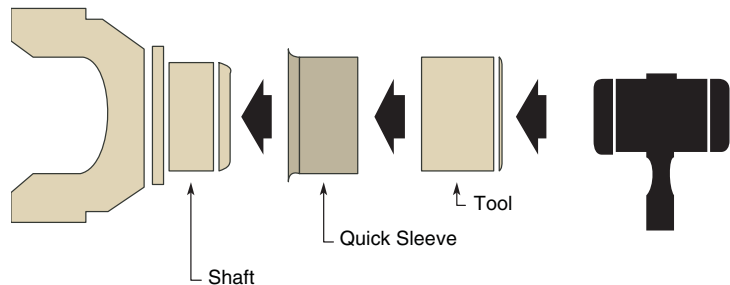
Quick Sleeve Installation
