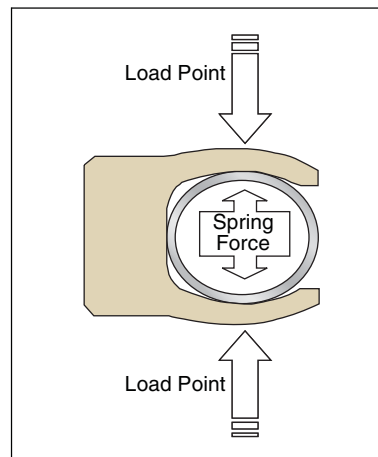
Figure 2-17. Installed State
