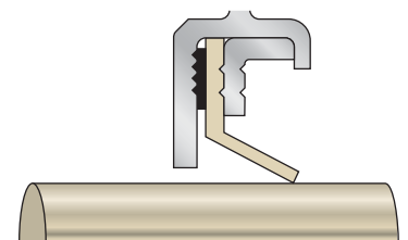
Machined Lip
