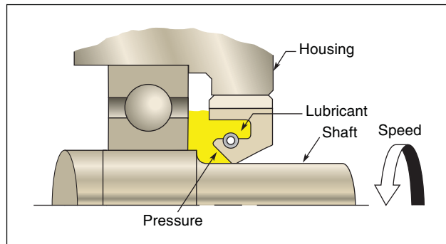
Figure 2-5. Sealing System
