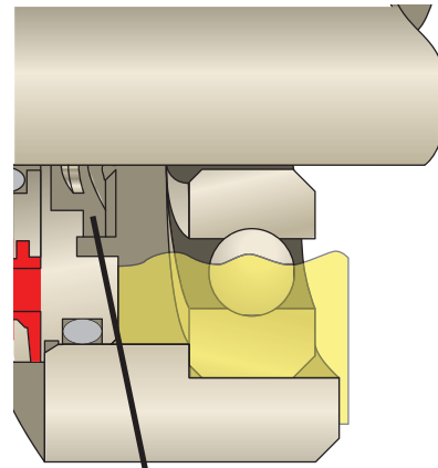
Severe Splash Groove
