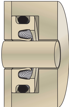
Rotary Housing
