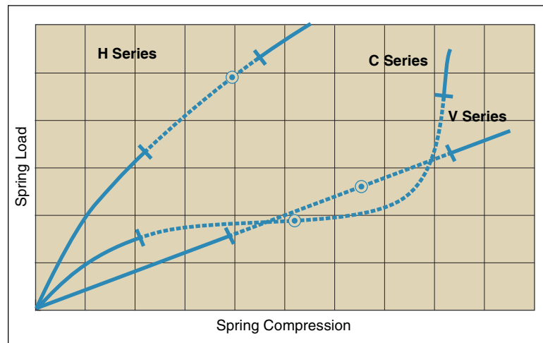
Figure 2-14. FlexiSeal Spring Energizers
