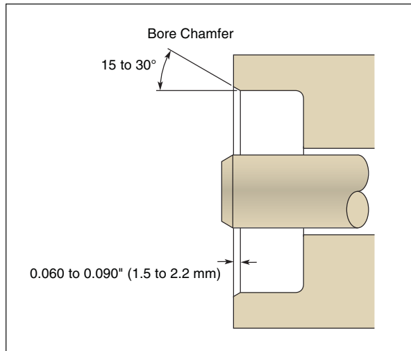
Figure 5-2. Housing Profile
