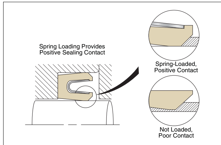
Figure 2-13. Spring Loading
